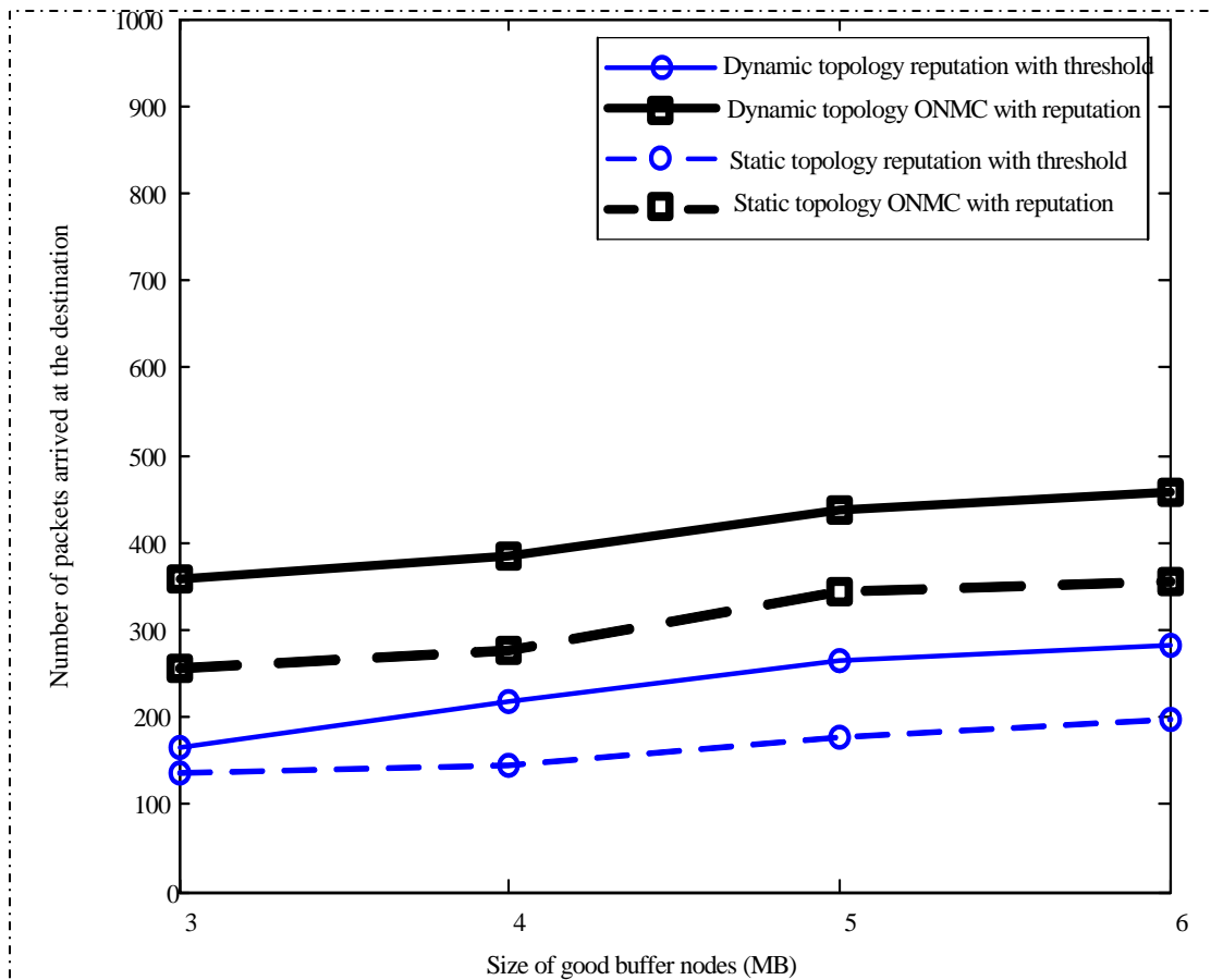
Figure 4.9 Effect of varying the buffer size of good nodes with n_m=1000 .
